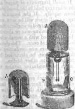
FIG. 2.—Cavallo's Electroscopes.
