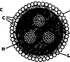
FIG. 7.—Triple Conductor Armoured Cable (Section).
