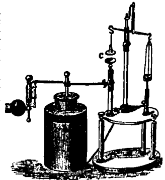
FIG. 1.—Snow-Harris's Disk Electrometer.
