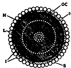
FIG. 6.—Armoured Concentric Cable (Section).
