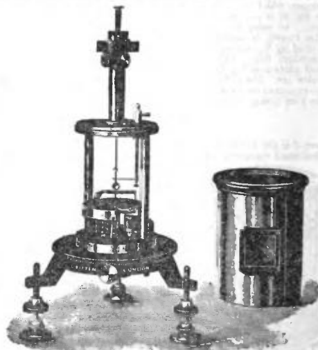
FIG. 7.—Quadrant Electrometer. Dolezalek Pattern.
