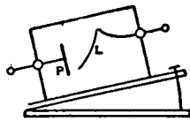
FIG. 7.—Wilson's Electroscope.
