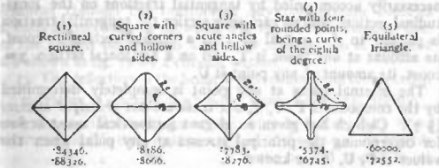
FIG. 8.—Diagrams showing Torsional Rigidities.
